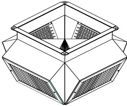
Model DSFD with Double Deflection Grilles 4-Way Discharge
